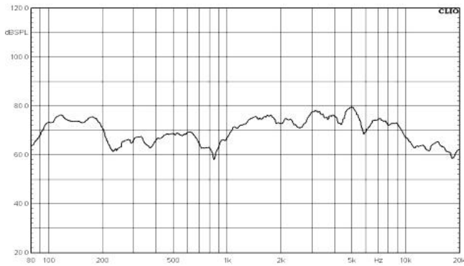
Frequency Response
